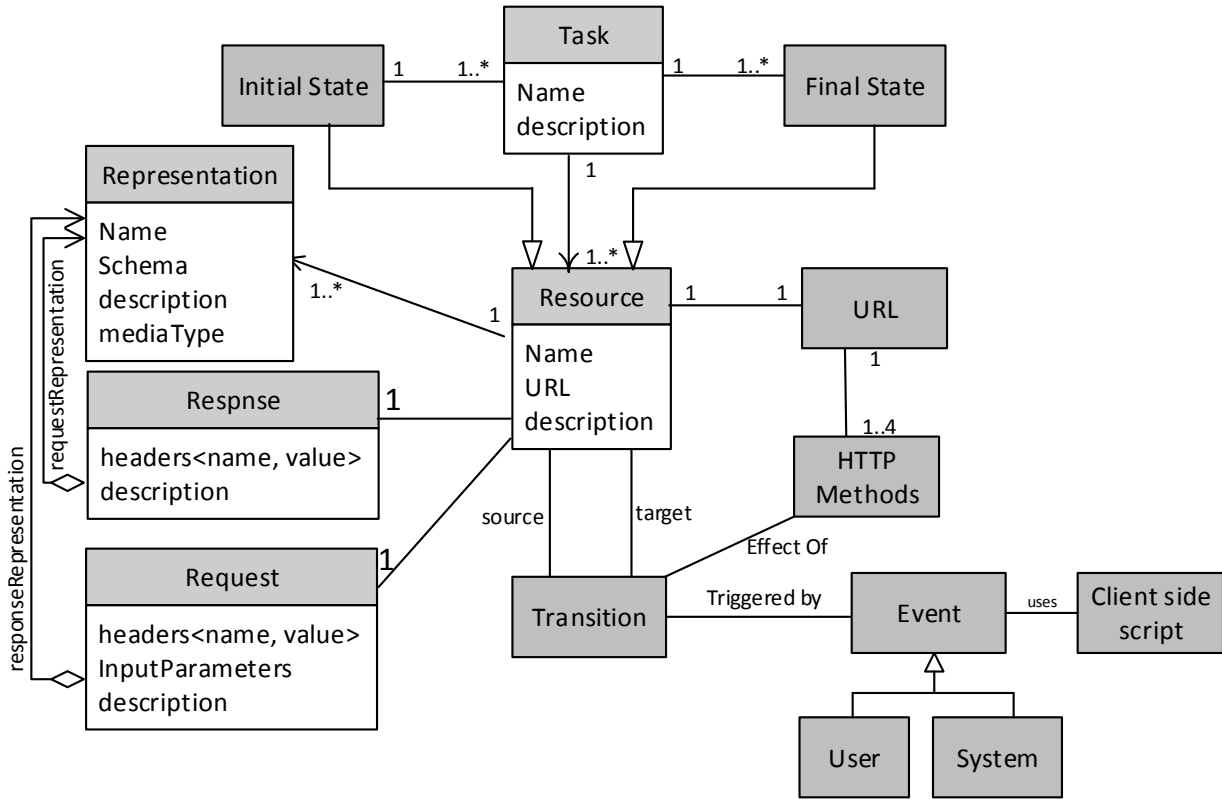
Figure 2: Meta-model for users' tasks
