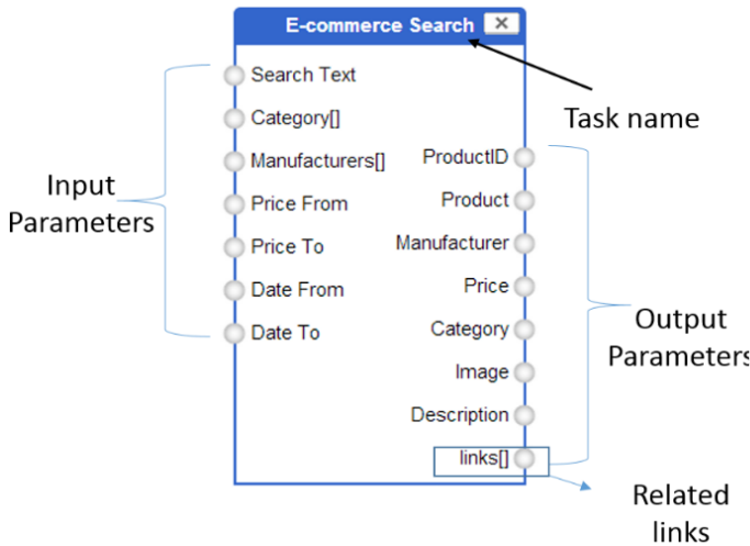
Figure 8: A task showing input parameters, output parameters and related links
