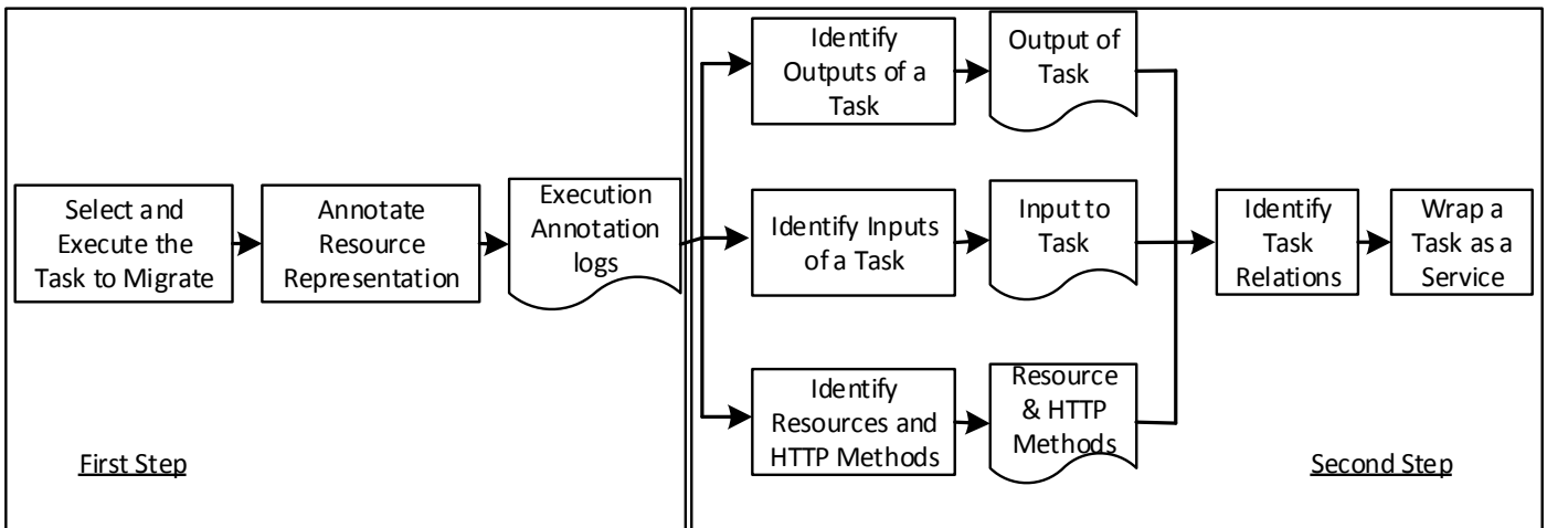
Figure 3: Overview of our approach to identify services from a web page
