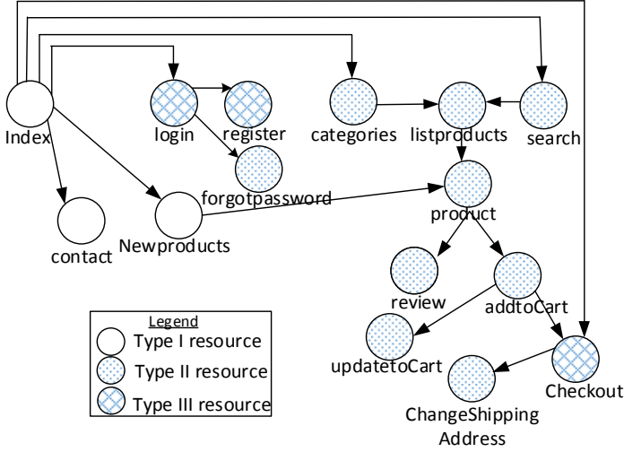
Figure 7: Task relations extracted from a web application in E-commerce domain
